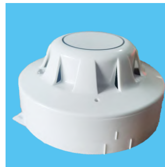
SMOKE DETECTOR Model DFS516 Operated volt-9VDC-35VDC; Sensor:Optical sensor; Sensitivity-0.15 dB/m( \pm 0.03 dB/m); Standby current: \leq 50\mu A (2 wires); Alarm current: \leq 50mA ;
